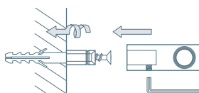
HG18-50D Wandmontage:
